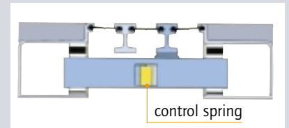
Opened joint, cross-section
